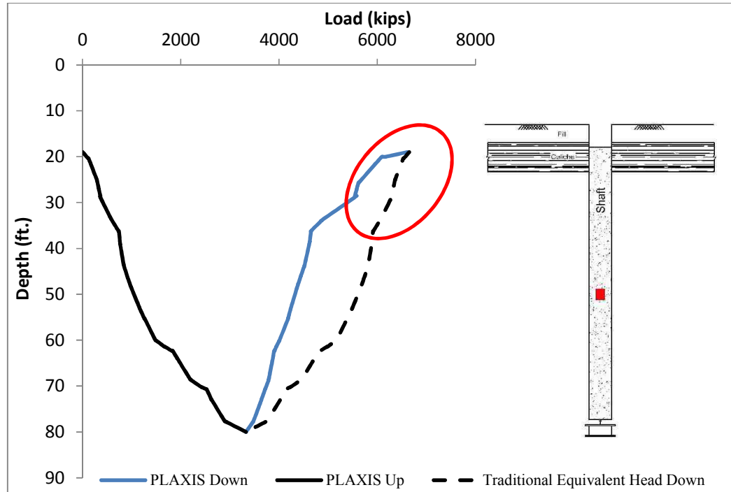
Figure 6-5: Load Transfer
